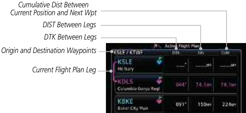
Figure 4-31 Flight Plan Data Fields
