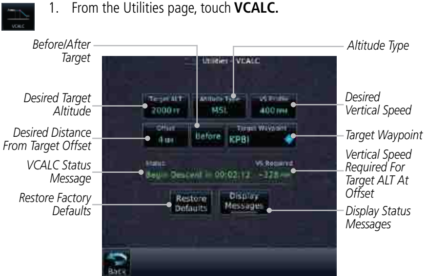
Figure 15-5 VCALC Page
